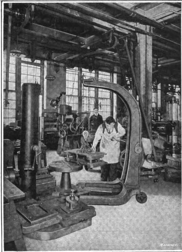
Fig. 3—In setting up heavy pieces on machine tools, it may be difficult to handle work on a traveling crane, due to the inability of that kind of equipment to reach the desired point. This illustration shows a view in the Cadillac Motor Car Co.'s factory, where a portable crane built by the Franklin Machine Works, Franklin, Pa., is engaged in setting up work on the table of a radial drilling machine
